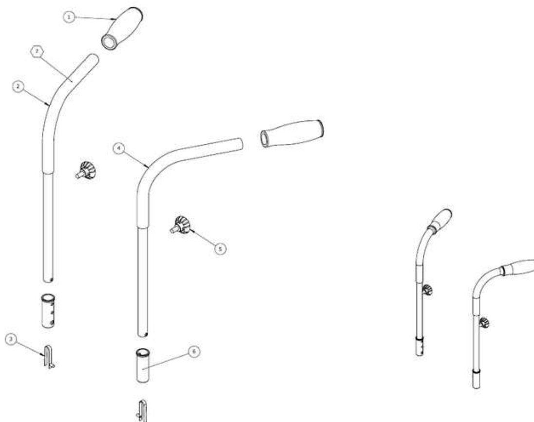
Item numbers Push handles, set (95370-10)
