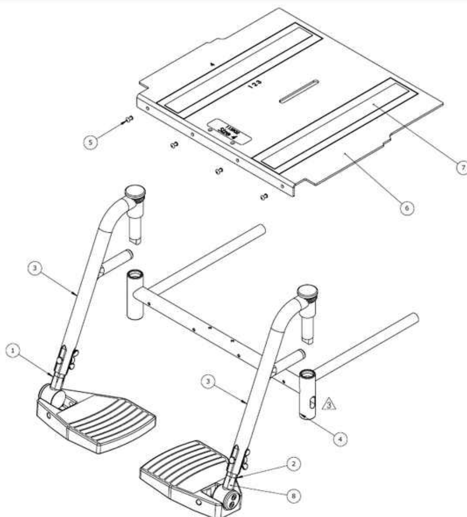
Item numbers for Foot rests, parted, size 3 (95151-360) size 4 (95151-460)
