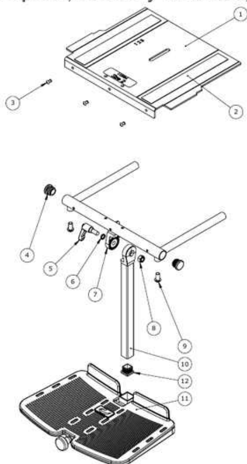
Item numbers for Foot plate, centrally mounted, size 1 (95152-160), size 2 (95152-260)
