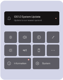
Software Upgrades
