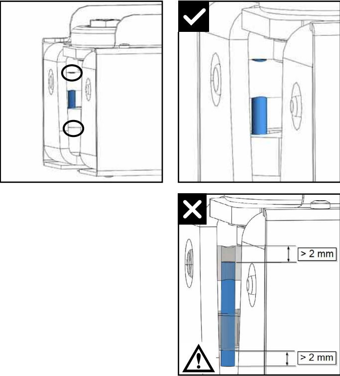
Figure 4 Visually inspect the pins inside the coupling. If difficult to inspect apply a torch, camera or engage the mechanism. The pin top should be flush with the axle surface. If a pin is not flush (+/- 2 mm is acceptable) the coupling must be taken out of service until a service technician has inspected the coupling.
