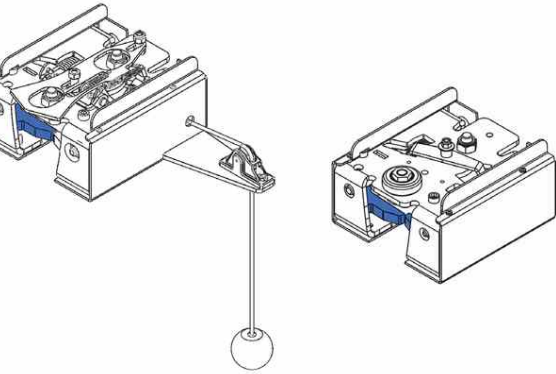
Figure 3 Height from pulley (knob) to ground is min. 1.8 m.
