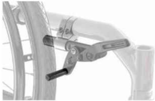
WL08 ↑ Newton wheel lock – push to lock
